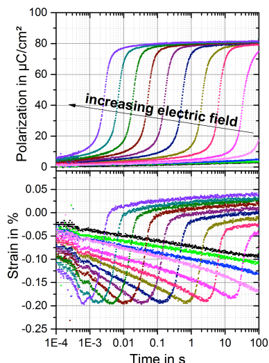
Figure 1: Simultaneous measurement of polarization and strain dynamics at various fields (0.5kV/mm–1.2kV/mm) for rhombohedral \text{Pb}(\text{Zr},\text{Ti})\text{O}_3 polycrystalline ceramic.
